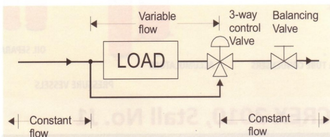
Figure 1 : Schematic of a control valve and a balancing valve in a constant flow system
